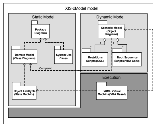
Fig. 4. Model organization for testing scenarios for simulation and animation.
