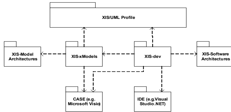
Fig. 2. ProjectIT-MDD (XIS) Overview.
