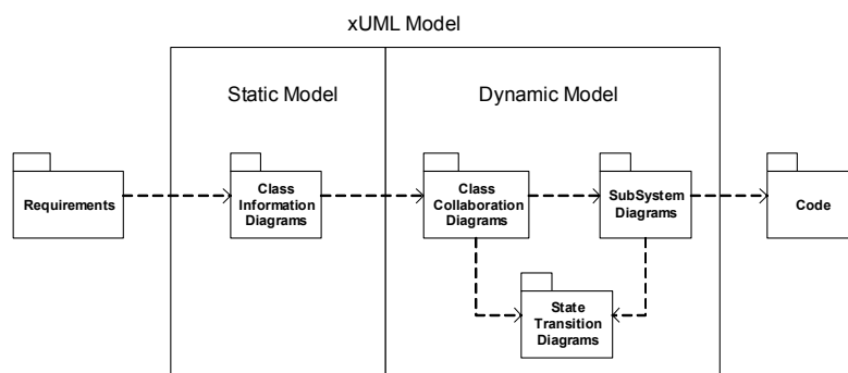
Fig. 1. xUML model components.
