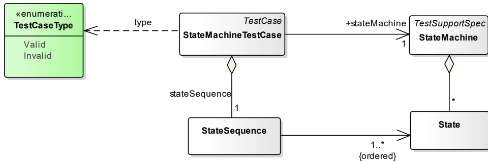
Figure 4: Metamodel of the TSL StateMachineTestCase definition (partial view).
