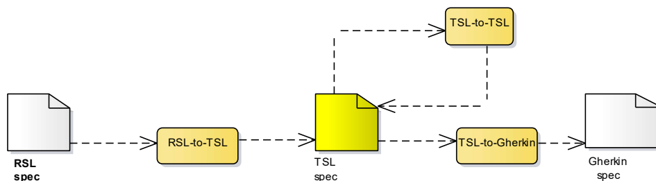
Figure 1: TSL based approach.
