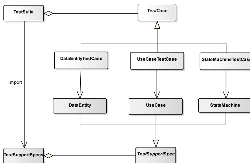
Figure 2: Metamodel of the TSL general architecture (partial view).
