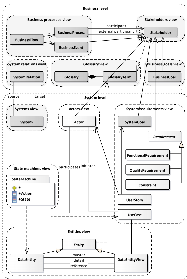
Figure 1: RSL metamodel (simplified). The constructs in dark grey background are applied in the scope of this paper.
