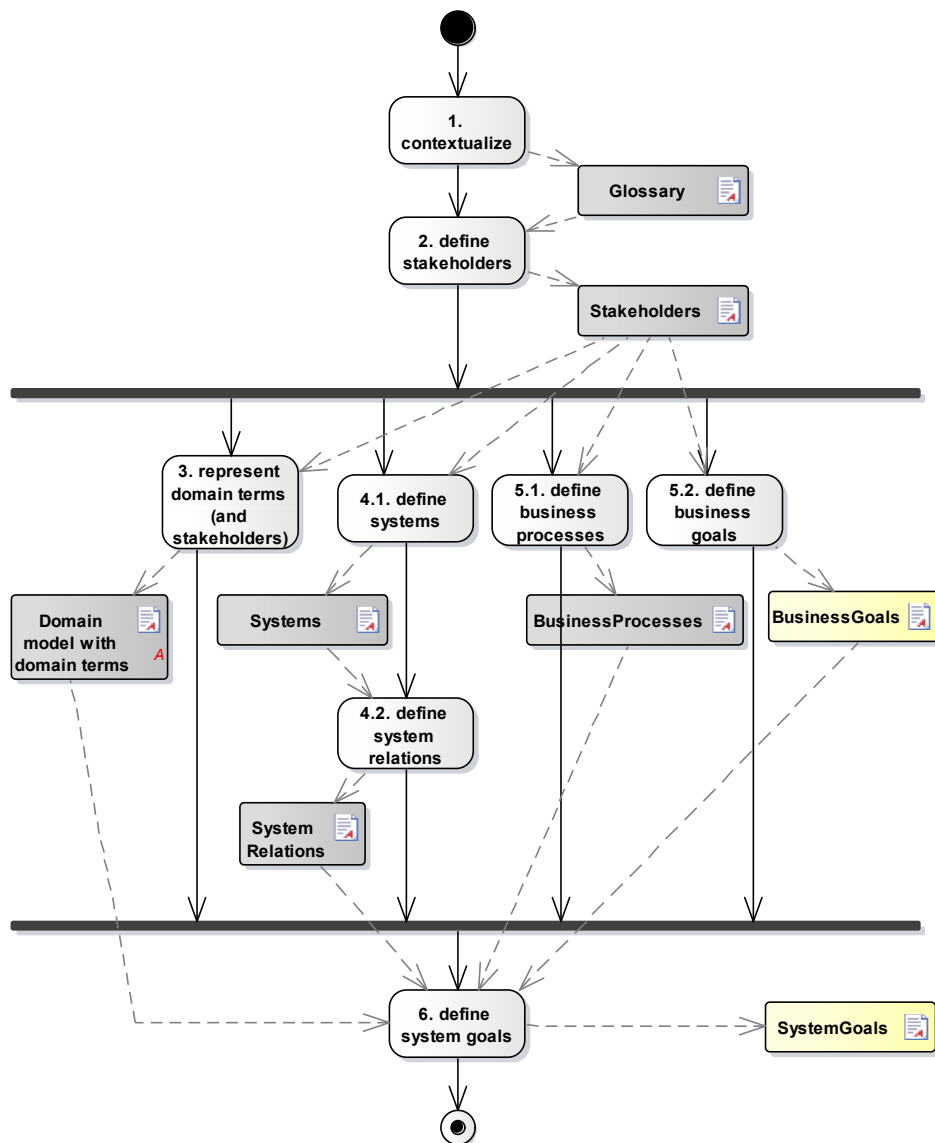
Figure 3: Methodology for analysing the GDPR.
